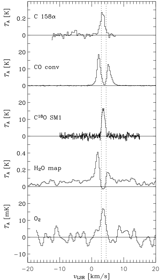
Fig. 2. The Hanning-smoothed O_2 line spectrum is shown in the bottom panel and compared to Odin H_2O ( 1_{1,0}-1_{0,1} ) line data (Larsson et al. 2007), to C^{18}O (3–2) and CO (3–2) from the JCMT-archive, and the C 158 \alpha recombination line from Pankonin & Walmsley (1978). The H_2O spectrum represents the average of the part of the \rho Oph A cloud mapped with Odin (slightly larger than 5' \times 4' ). The C^{18}O spectrum (15'' beam) refers to a pointed observation toward the Odin center coordinates, while the CO spectrum is that of the 3.5' \times 10' (at PA = 45^\circ ) CO (3–2) map convolved with the 10' Odin beam. The displayed spectrum of the C 158 \alpha recombination line refers to the average of 4 map positions covering about 10' \times 10' . Vertical dotted lines are shown at v_{\text{LSR}} = +3.0 \text{ km s}^{-1} and +4.5 \text{ km s}^{-1} , respectively.
