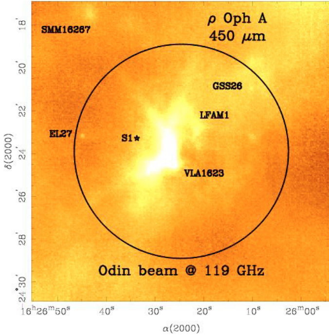
Fig. 1. The 10' Odin beam at 119 GHz, the frequency of O_2 ( N_J = 1_1-1_0 ), is shown as the large circle superposed onto the 450 \mu\text{m} map by Hargreaves (2004, see also Wilson et al. 1999). At the distance of 145 pc (de Zeeuw et al. 1999), the beam size corresponds to 0.4 pc. A few discrete sources are labelled. The observations were centered on RA = 16^{\text{h}}26^{\text{m}}24^{\text{s}}.6 , Dec = -24^{\circ}23'54'' (J2000).
