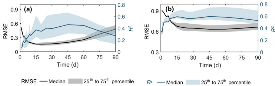
Fig. 2 Estimating the acclimation time scale of leaf respiration. The relationship ( R^2 and root mean square error (RMSE)) of doymean R_{d,25} observations to R_{d,25} predictions according to H4 for different numbers of prior days, derived from (a) the B4WarmED dataset and (b) the combined GlobResp and leaf carbon exchange (LCE) dataset.
